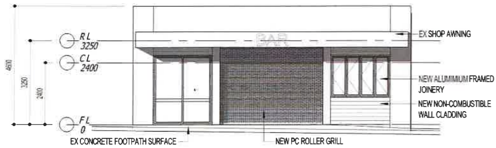
1 elevation to south 1:100
