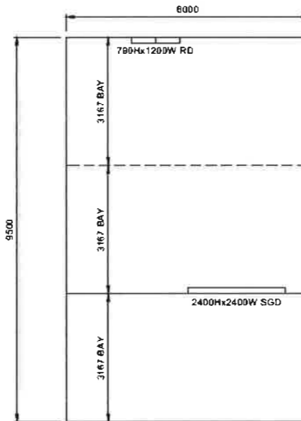
Mezzanine Floor Plan
