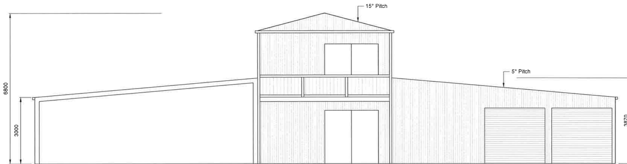
Front Elevation
