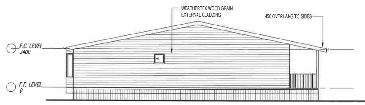
3 elevation to east 1 : 100
