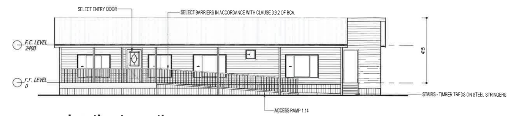
4 elevation to north 1 : 100
