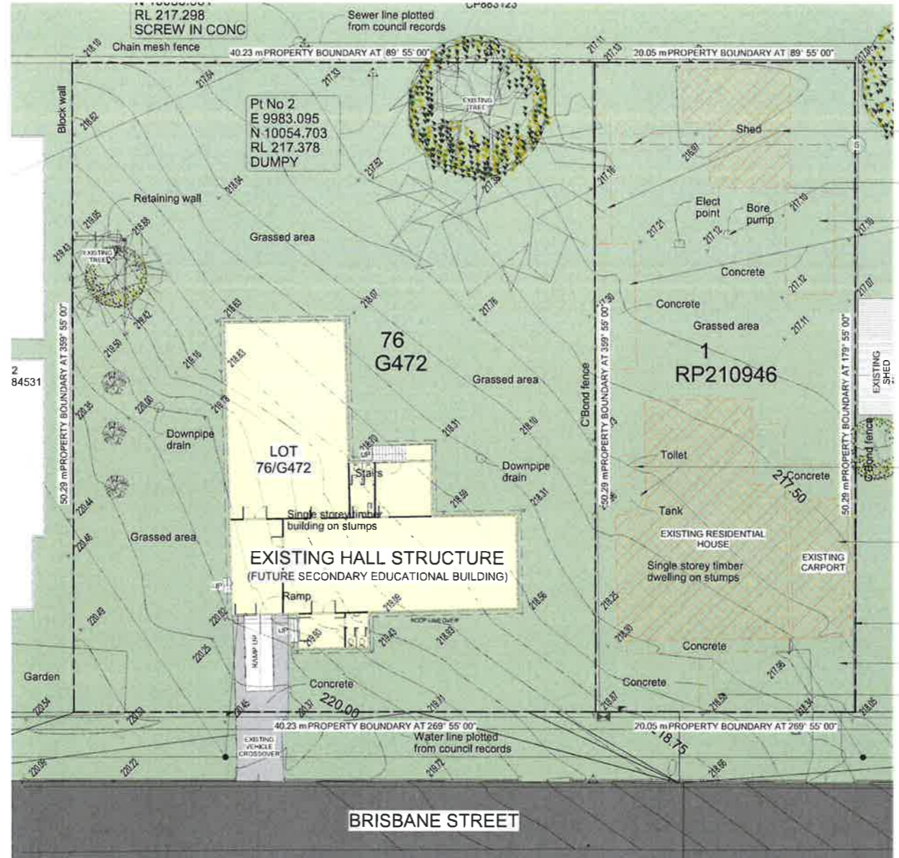
1 Existing/Demo Site Plan 1 : 200
