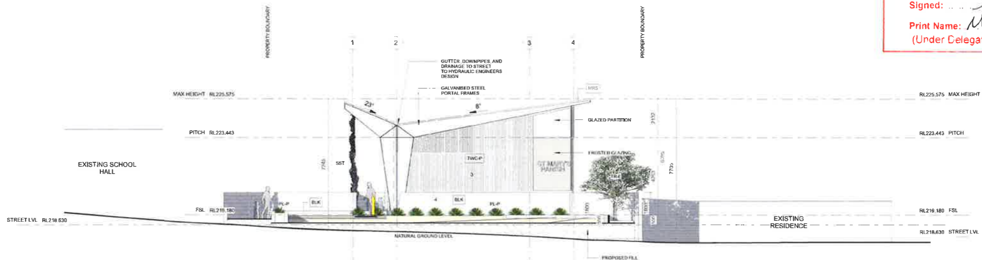
1 South Elevation 1 : 100
