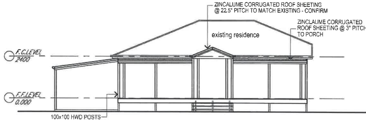
elevation to west
