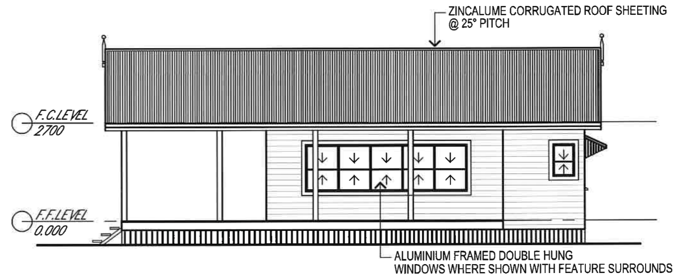
elevation to north-west
