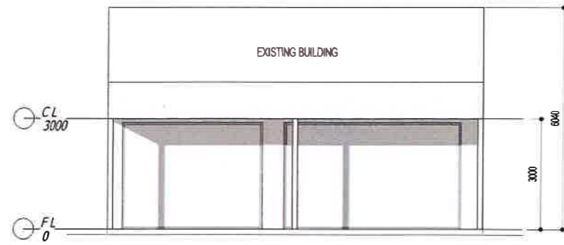
1 elevation to south 1:100
