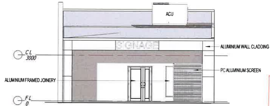
2 elevation to north 1:100
